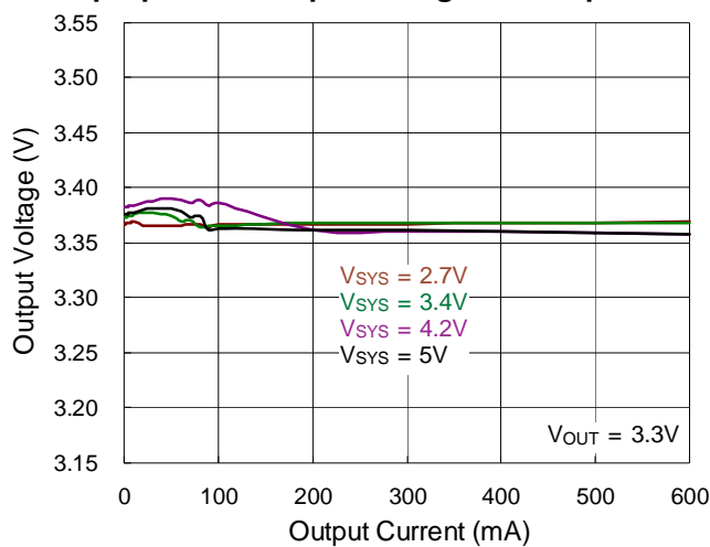
CH2 Step-Up/Down Output Voltage vs. Output Current
